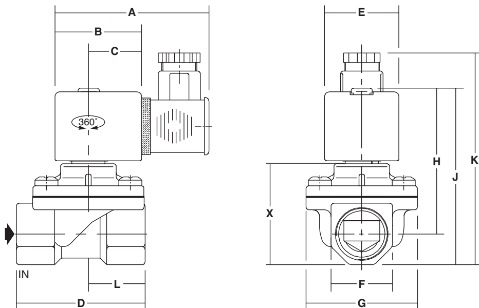
TYPE 01 Prefix "SC" Solenoid Epoxy moulded IEC 335 / ISO 4400 IP65
