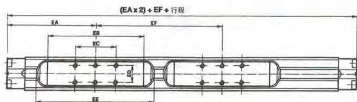
S1双中号滑台尺寸
