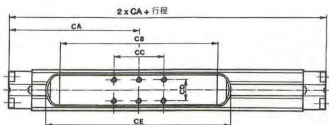
S1中号滑台尺寸
